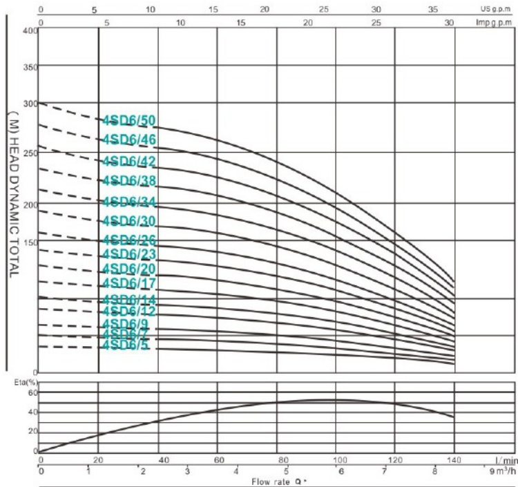
4SD(M)6 PERFORMANCE DATA 50Hz
