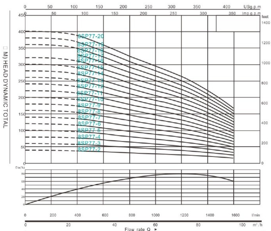
8SP77 PERFORMANCE DATA 50Hz
