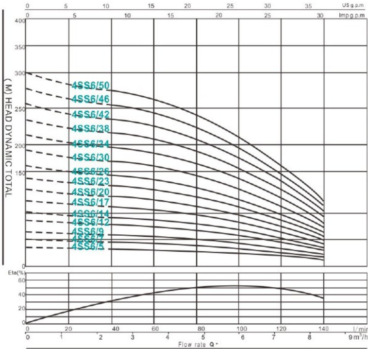
4SS(M)6 PERFORMANCE DATA 50Hz
