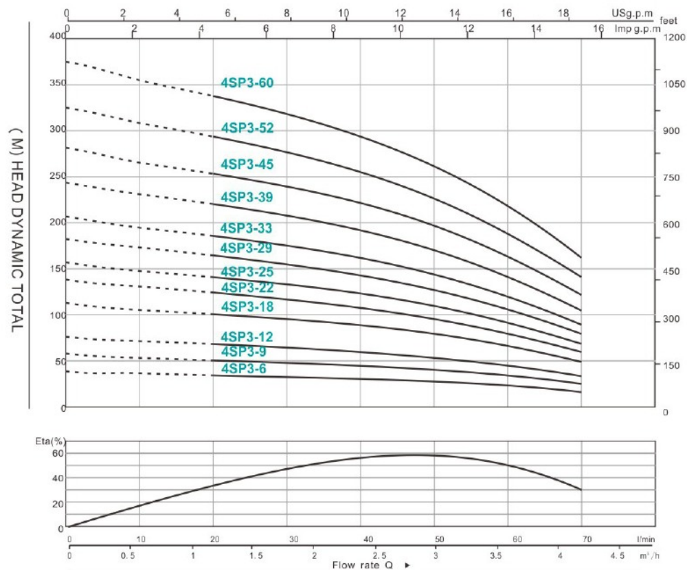
4SP(M)3 PERFORMANCE DATA 50Hz
