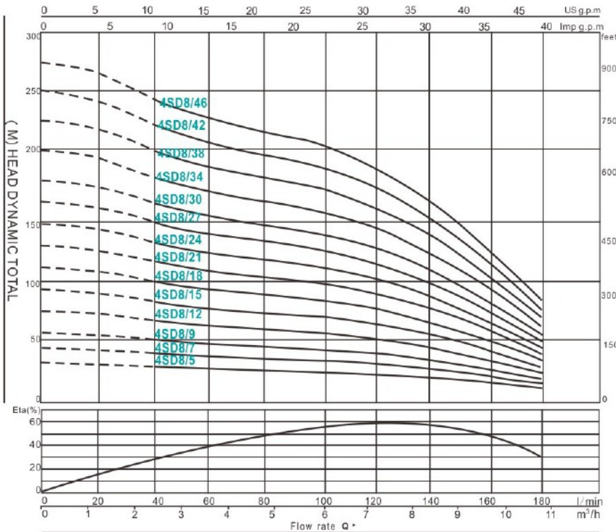
4SD(M)8 PERFORMANCE DATA 50Hz
