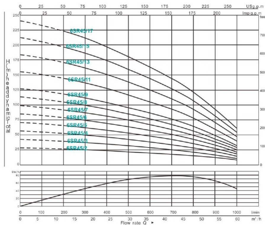
6SR(M)45 PERFORMANCE DATA 50Hz
