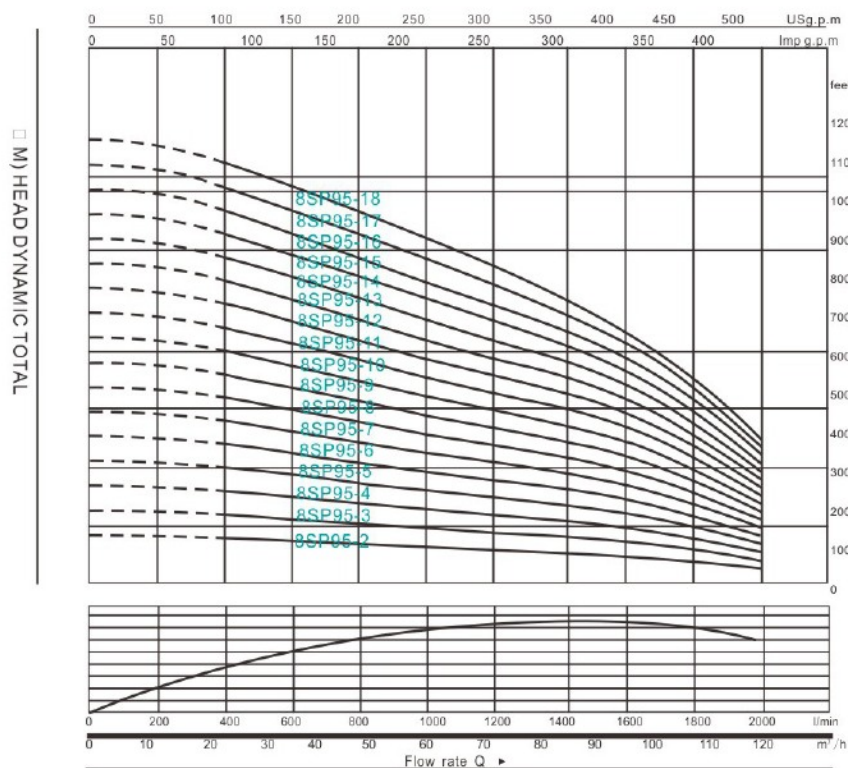
8SP95 PERFORMANCE DATA 50Hz
