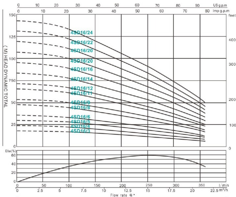
4SD(M)16 PERFORMANCE DATA 50Hz
