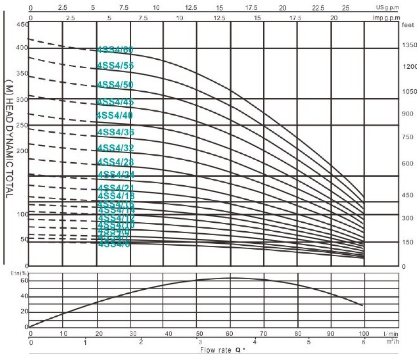
4SS(M)4 PERFORMANCE DATA 50Hz
