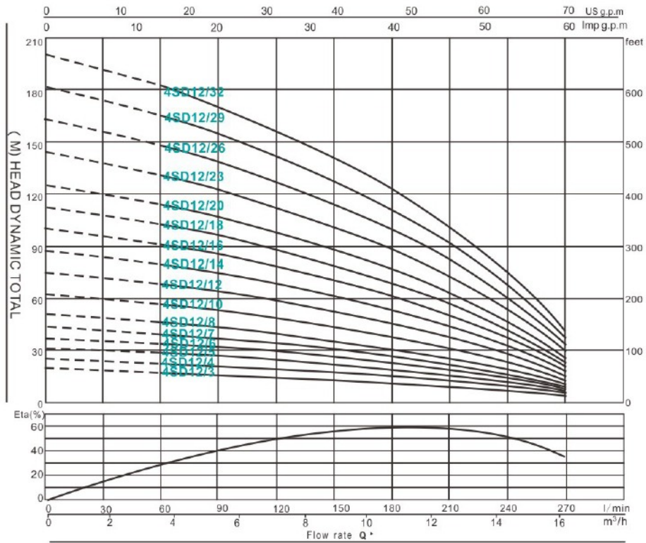
4SD(M)12 PERFORMANCE DATA 50Hz
