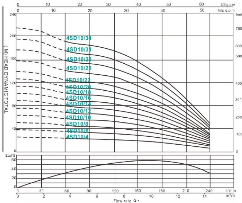
4SD(M)10 PERFORMANCE DATA 50Hz
